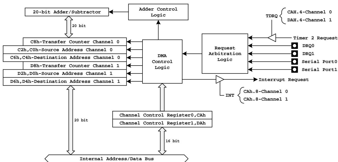
DMA Unit Block
