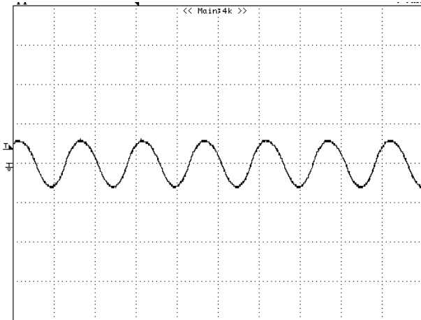
Figure 17: Input Terminal Ripple Current- i_c , at full rated output current and nominal input voltage with 12\mu\text{H} source impedance and 33\mu\text{F} electrolytic capacitor (500 mA/div, 2\mu\text{s}/\text{div} ).
