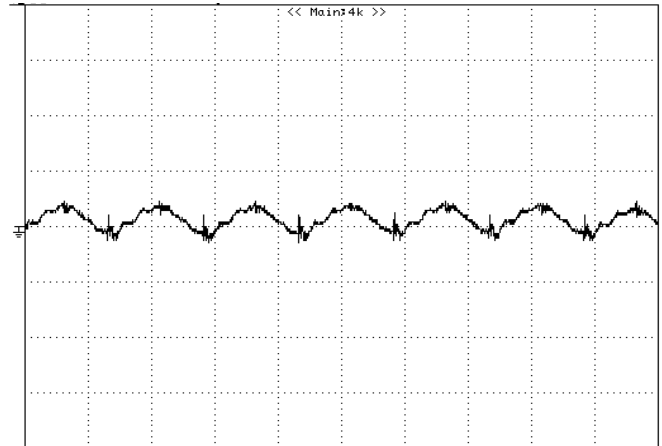
Figure 18: Input reflected ripple current- i_s , through a 12\mu\text{H} source inductor at nominal input voltage and rated load current (20 mA/div, 2\mu\text{s}/\text{div} ).
