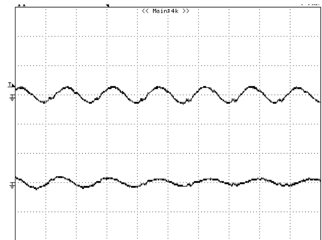
Figure 20: Output voltage ripple at nominal input voltage and rated load current ( I_{out1}=I_{out2}=\text{Full} ) (20 mV/div, 1\mu\text{s}/\text{div} ). Top trace: Vout2 (50mV/div), Bottom trace: Vout1(50mV/div) Load capacitance: 1\mu\text{F} ceramic capacitor and 10\mu\text{F} tantalum capacitor. Bandwidth: 20 MHz. Scope measurements should be made using a BNC cable (length shorter than 20 inches). Position the load between 51 mm to 76 mm (2 inches to 3 inches) from the module.
