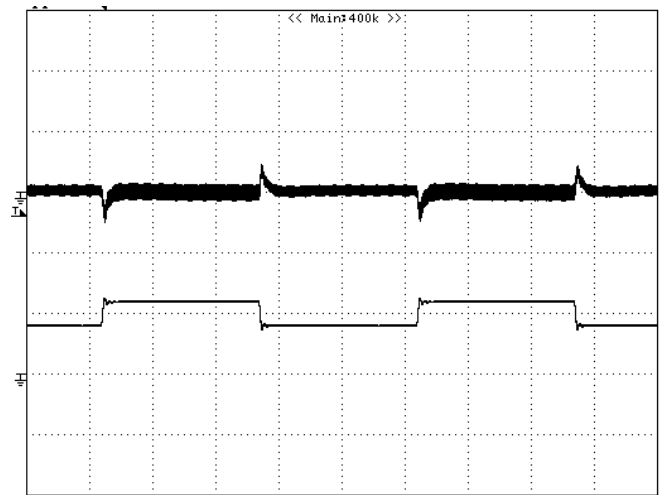
Figure 14: Output voltage response to step-change in load current lout1 (75%-50%-75% of I_o , max; di/dt = 2.5A/\mu s ) at lout2=0A, Load cap: 470 \mu F , 35m \Omega ESR solid electrolytic capacitor and 1 \mu F ceramic capacitor. Ch1=Vout1 (100mV/div), Ch2=lout1 (5A/div), Scope measurement should be made using a BNC cable (length shorter than 20 inches). Position the load between 51 mm to 76 mm (2 inches to 3 inches) from the module.
