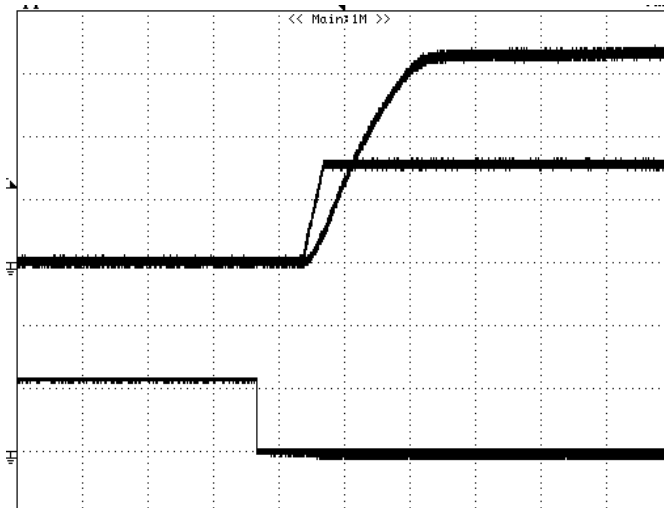
Figure 6: Turn-on transient at full rated load current (resistive load) (10 ms/div). V_{in}=48V . Negative logic turn on. Top Trace: Vout; 1V/div; Bottom Trace: ON/OFF input: 5V/div
