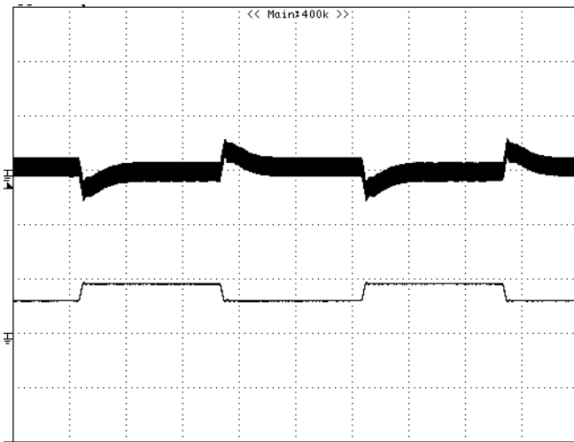
Figure 13: Output voltage response to step-change in load current lout2 (75%-50%-75% of I_o , max; di/dt = 2.5A/\mu s ) at lout1=0. Load cap: 470 \mu F , 35m \Omega ESR solid electrolytic capacitor and 1 \mu F ceramic capacitor. Ch1=Vout2 (100mV/div), Ch2=lout2 (5A/div), Scope measurement should be made using a BNC cable (length shorter than 20 inches). Position the load between 51 mm to 76 mm (2 inches to 3 inches) from the module.
