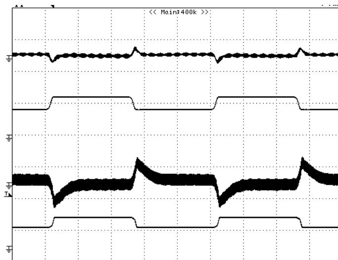
Figure 12: Output voltage response to step-change in load current lout2 and lout1 (75%-50%-75% of I_o , max; di/dt = 0.1A/\mu s ). Load cap: 10\mu F , tantalum capacitor and 1\mu F ceramic capacitor. Ch1=Vout1 (100mV/div), Ch2=lout1 (5A/div), Ch3=Vout2 (100mV/div), Ch4=lout2 (5A/div) Scope measurement should be made using a BNC cable (length shorter than 20 inches). Position the load between 51 mm to 76 mm (2 inches to 3 inches) from the module.
