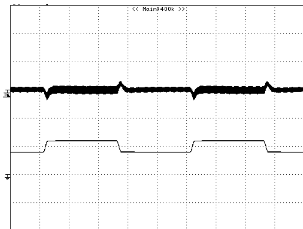
Figure 11: Output voltage response to step-change in load current lout1 (75%-50%-75% of I_o , max; di/dt = 0.1A/\mu s ) at lout2=0. Load cap: 10\mu F , tantalum capacitor and 1\mu F ceramic capacitor. Ch1=Vout1 (100mV/div), Ch2=lout1 (5A/div), Scope measurement should be made using a BNC cable (length shorter than 20 inches). Position the load between 51 mm to 76 mm (2 inches to 3 inches) from the module.
