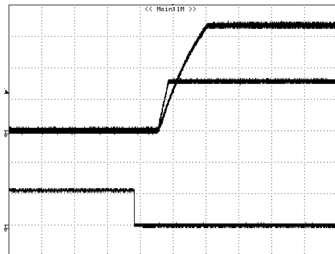
Figure 5: Turn-on transient at zero load current (10ms/div). V_{in}=48V . Negative logic turn on. Top Trace: Vout; 1V/div; Bottom Trace: ON/OFF input: 5V/div
