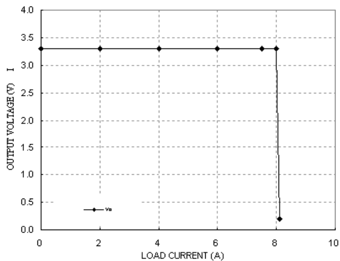
Figure 22: Output voltage vs. load current I_{out2} showing typical current limit curves and converter shutdown points.
