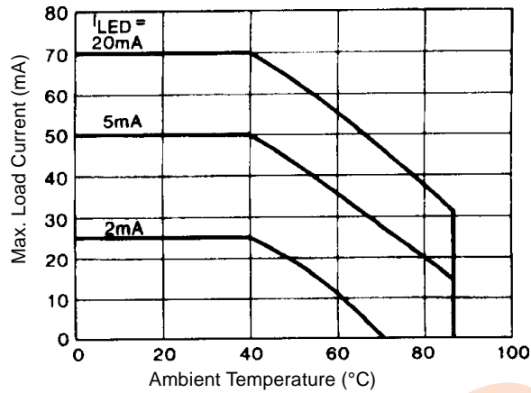
Figure 1. Current Derating Curves
