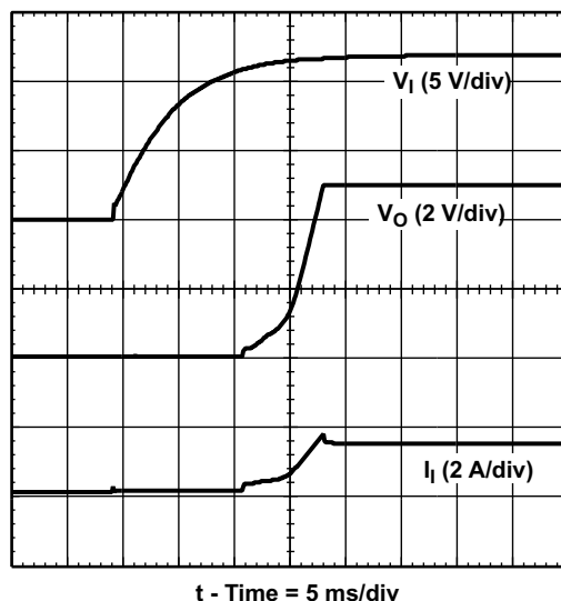
Figure 29. Power-Up Waveforms
