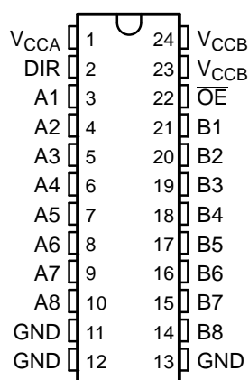
DB, DGV, OR PW PACKAGE (TOP VIEW)
