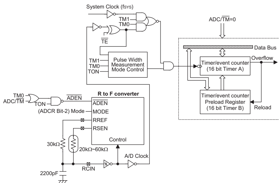
Timer/Event Counter
