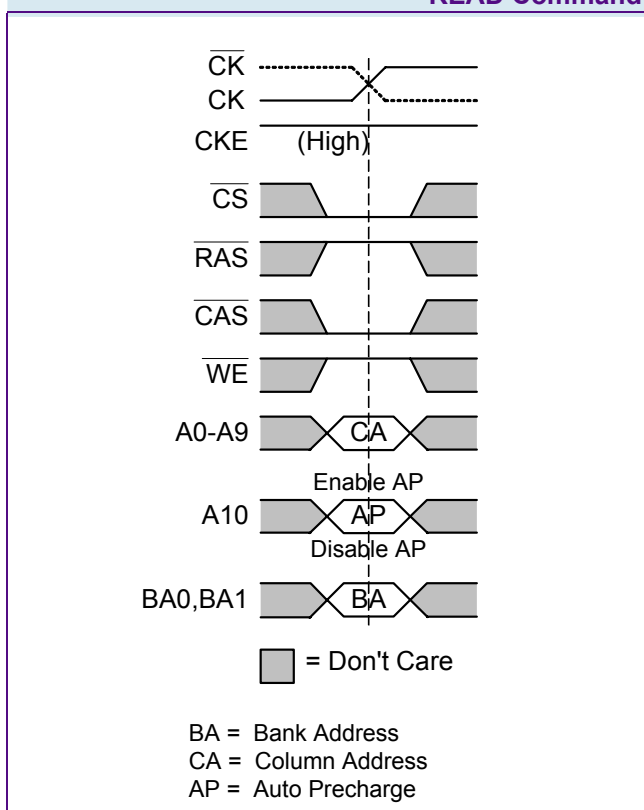
FIGURE 12 READ Command
