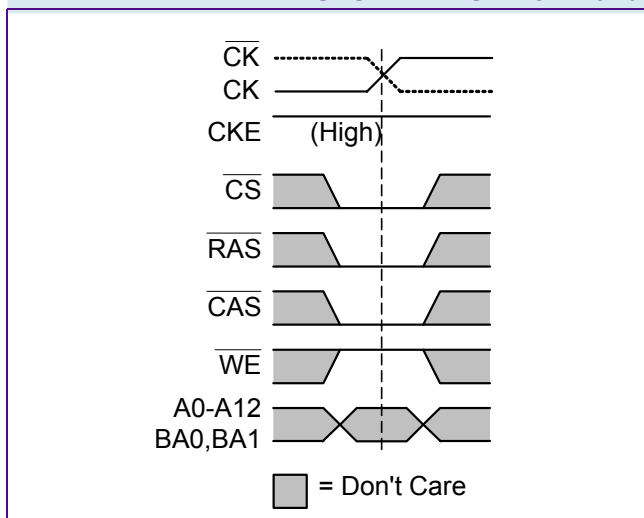
FIGURE 33 AUTO REFRESH Command
