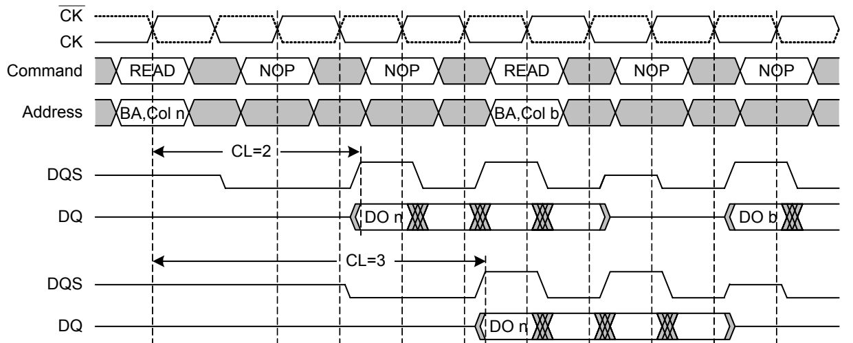
FIGURE 16 Nonconsecutive READ Bursts
