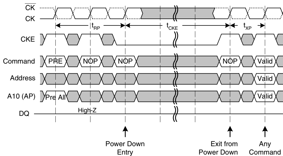
FIGURE 38 Power-Down Entry and Exit
