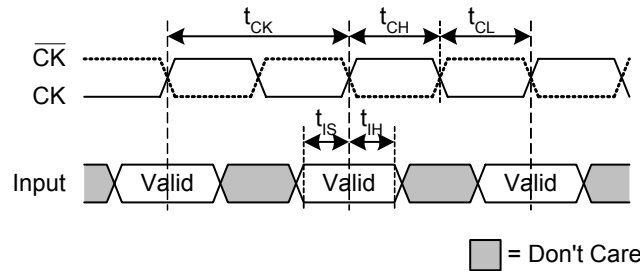
FIGURE 6 Address / Command Inputs Timing Parameters
