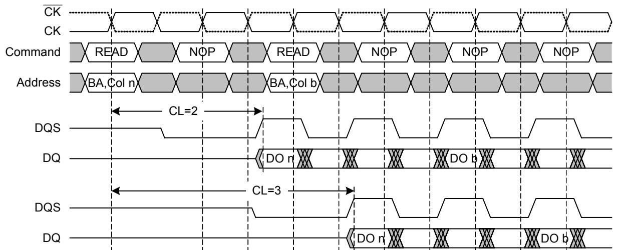
FIGURE 15 Consecutive READ Bursts
