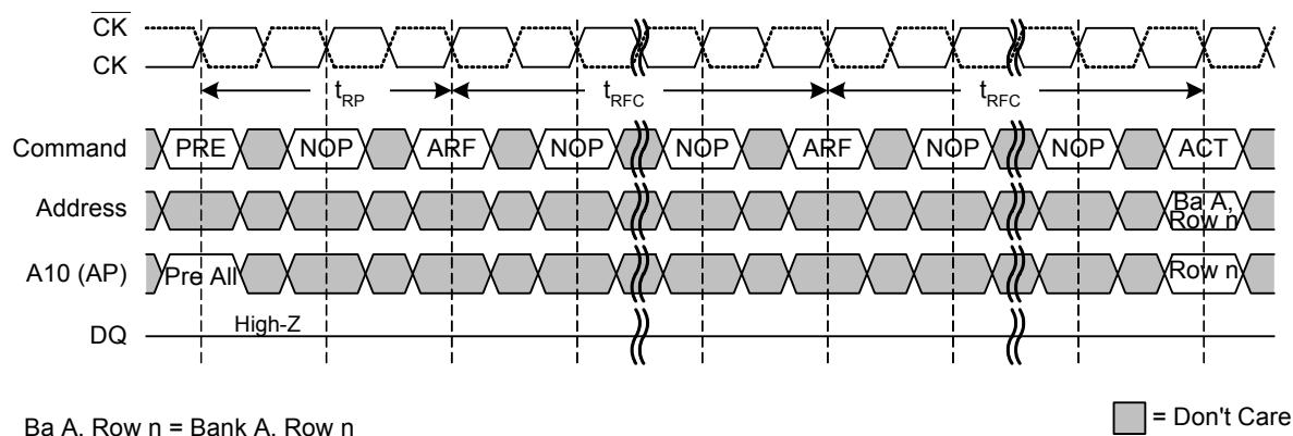
FIGURE 34 Auto Refresh
