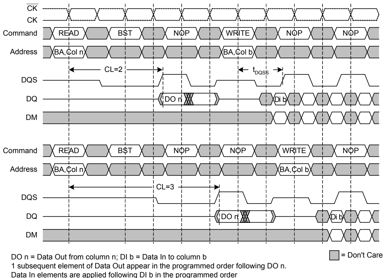
FIGURE 19 READ to WRITE
