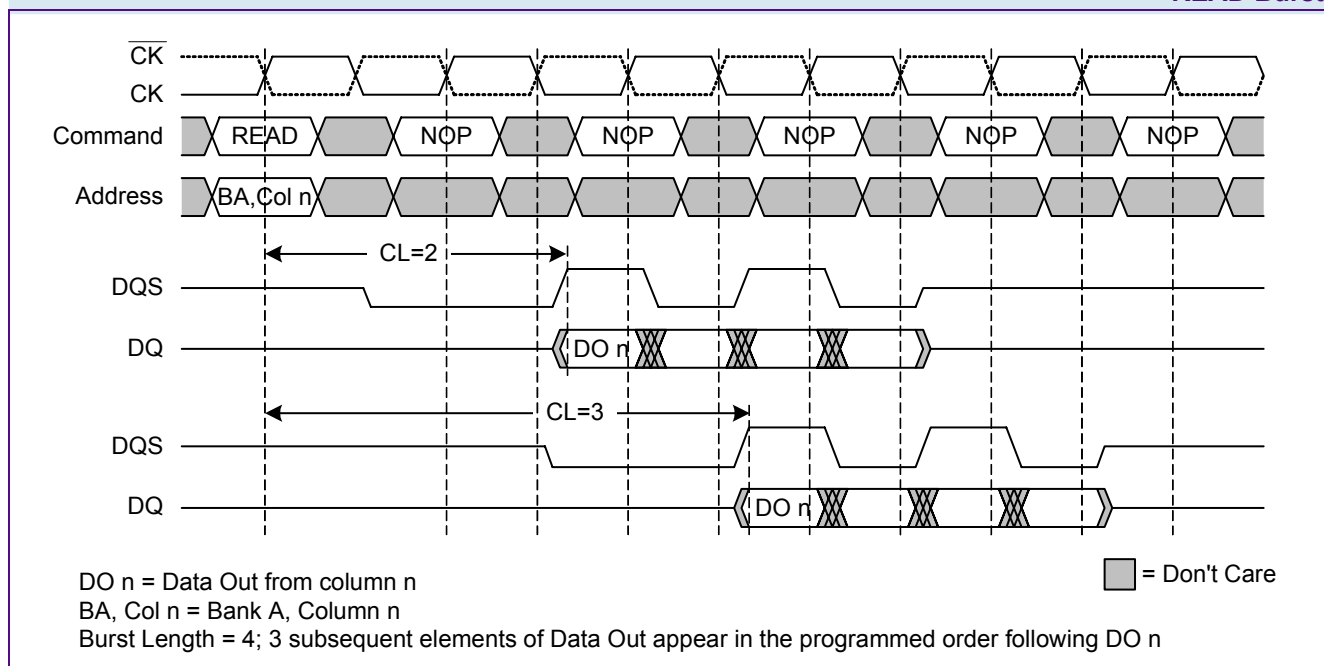
FIGURE 14 READ Burst
