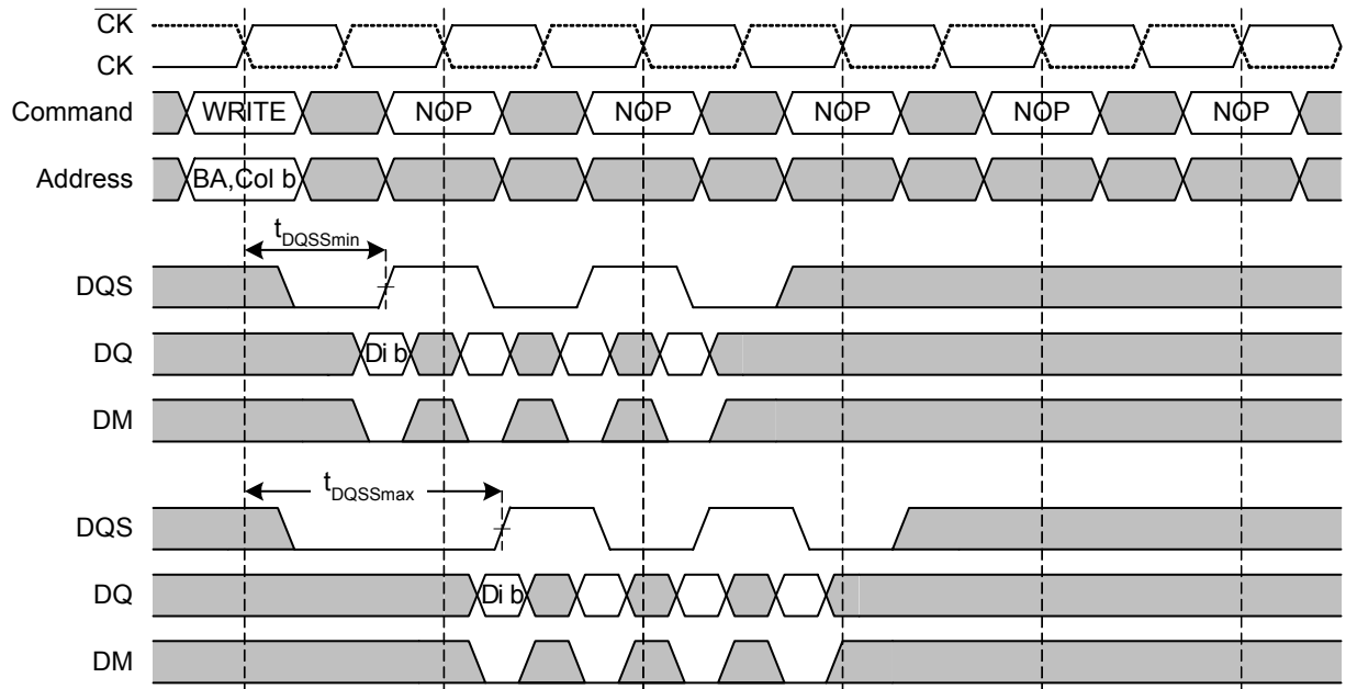
FIGURE 24 WRITE Burst (min. and max. t_{DQSS} )
