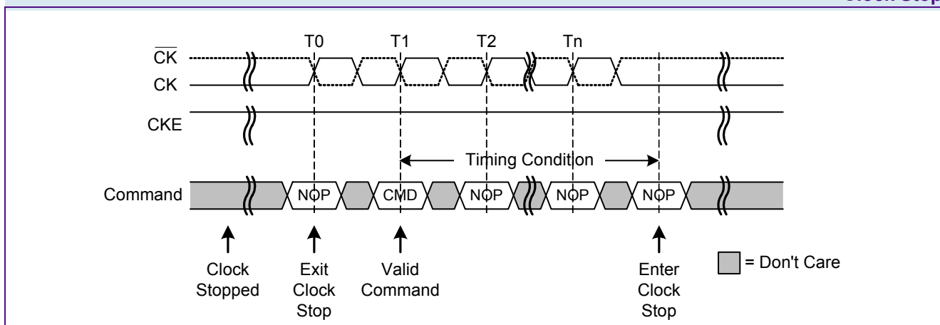
FIGURE 39 Clock Stop
