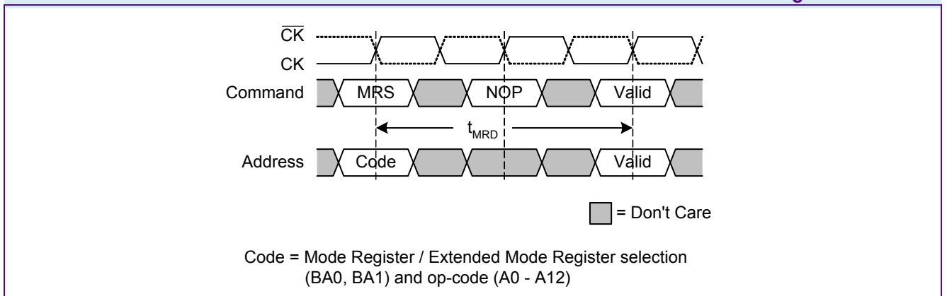
FIGURE 9 Mode Register Definition
