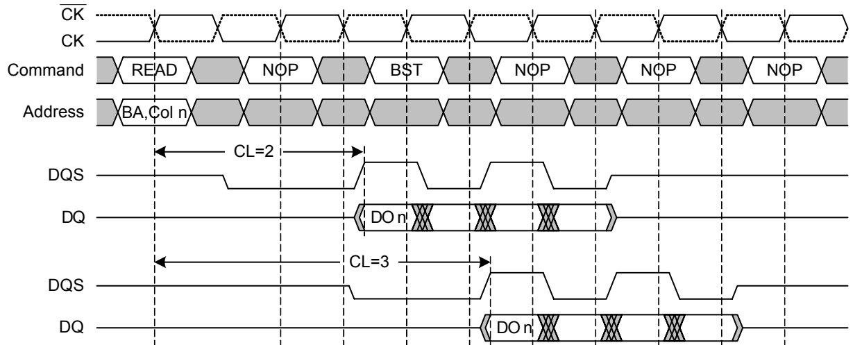
FIGURE 18 Terminating a READ Burst
