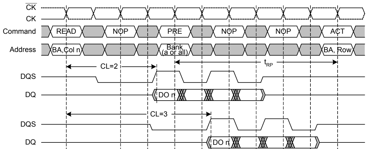
FIGURE 20 READ to PRECHARGE
