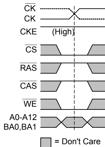
FIGURE 21 BURST TERMINATE Command
