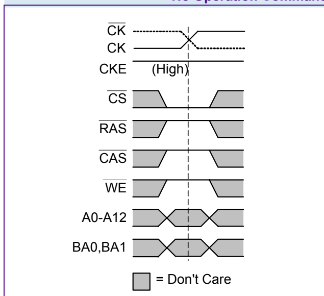
FIGURE 7 No Operation Command
