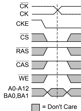
FIGURE 37 Power-Down Entry Command
