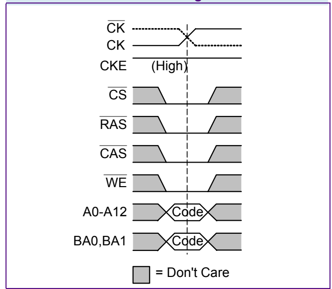
FIGURE 8 Mode Register Set Command
