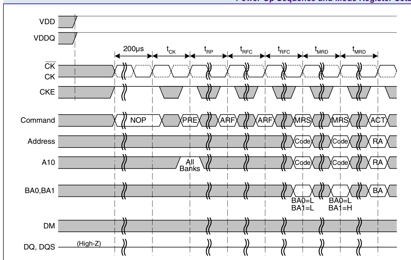
FIGURE 4 Power-Up Sequence and Mode Register Sets
