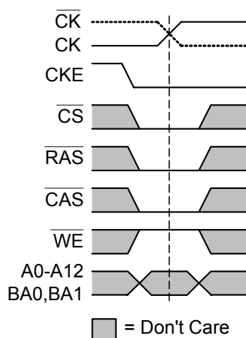
FIGURE 35 SELF REFRESH Entry Command
