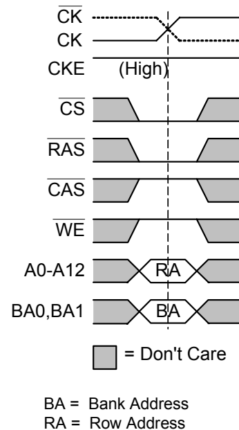
FIGURE 10 ACTIVE Command
