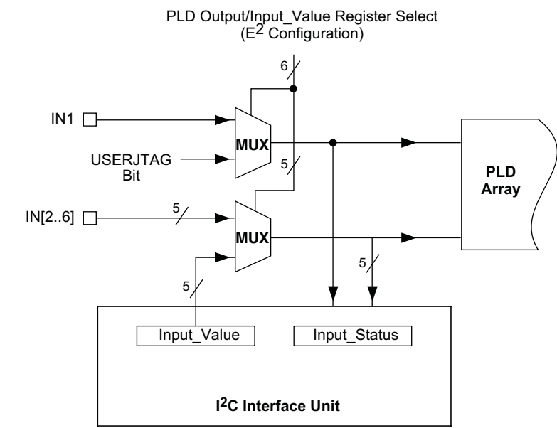
Figure 1-26. I 2 C Digital Input Interface
