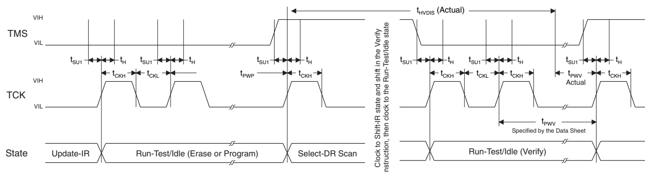
Figure 1-6. Discharge Timing Diagram
