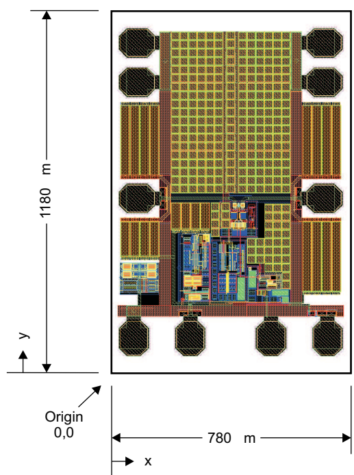
Figure 17. Chip Layout
