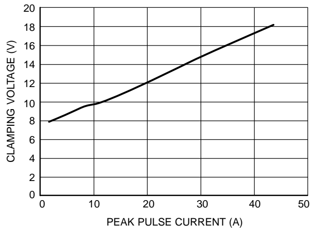
Figure 4. Clamping Voltage vs. Peak Pulse Current (8 × 20 \mu\text{s} Waveform)
