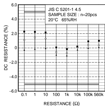
Fig.5 Resistance
