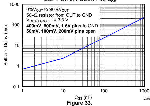
SOFT-START DELAY vs C_{SS}
