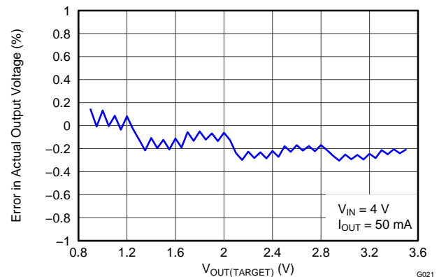
OUTPUT VOLTAGE: ACTUAL (Normalized) vs PIN-SETTING
