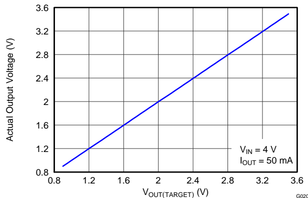
OUTPUT VOLTAGE: ACTUAL vs PIN-SETTING
