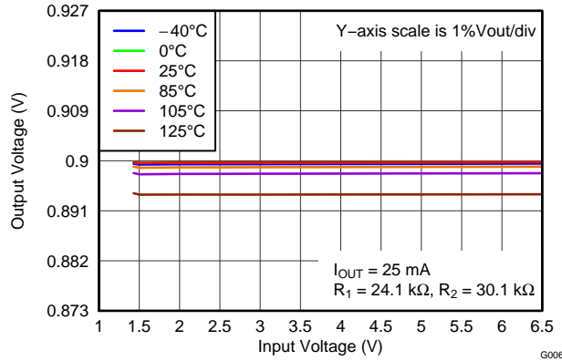
LINE REGULATION (0.9 V, Adjustable)
