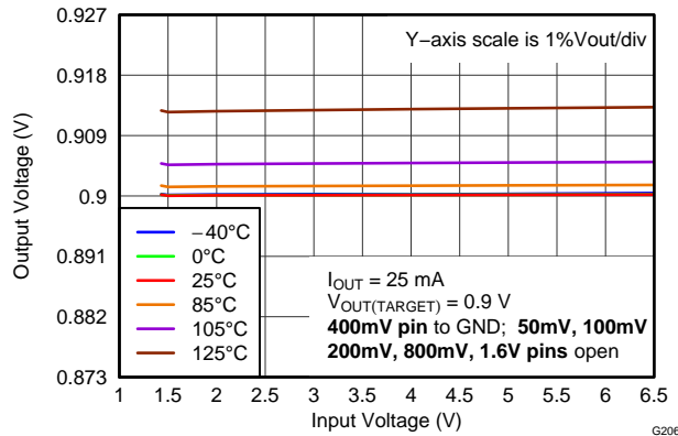
LINE REGULATION (0.9 V, Fixed by Setting Pins)
