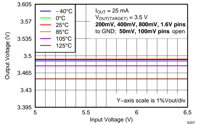
LINE REGULATION (3.5 V, Fixed by Setting Pins)
