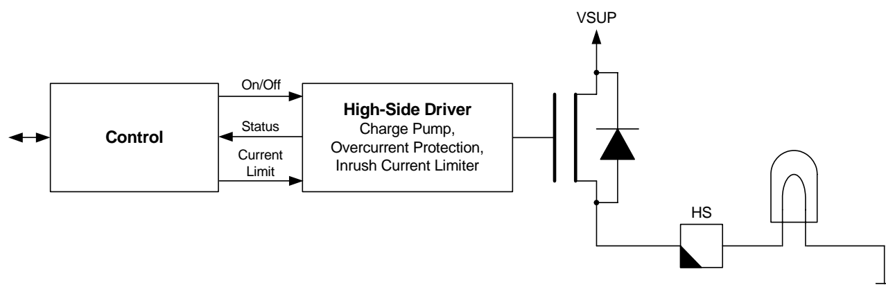
Figure 21. High-Side Circuitry
