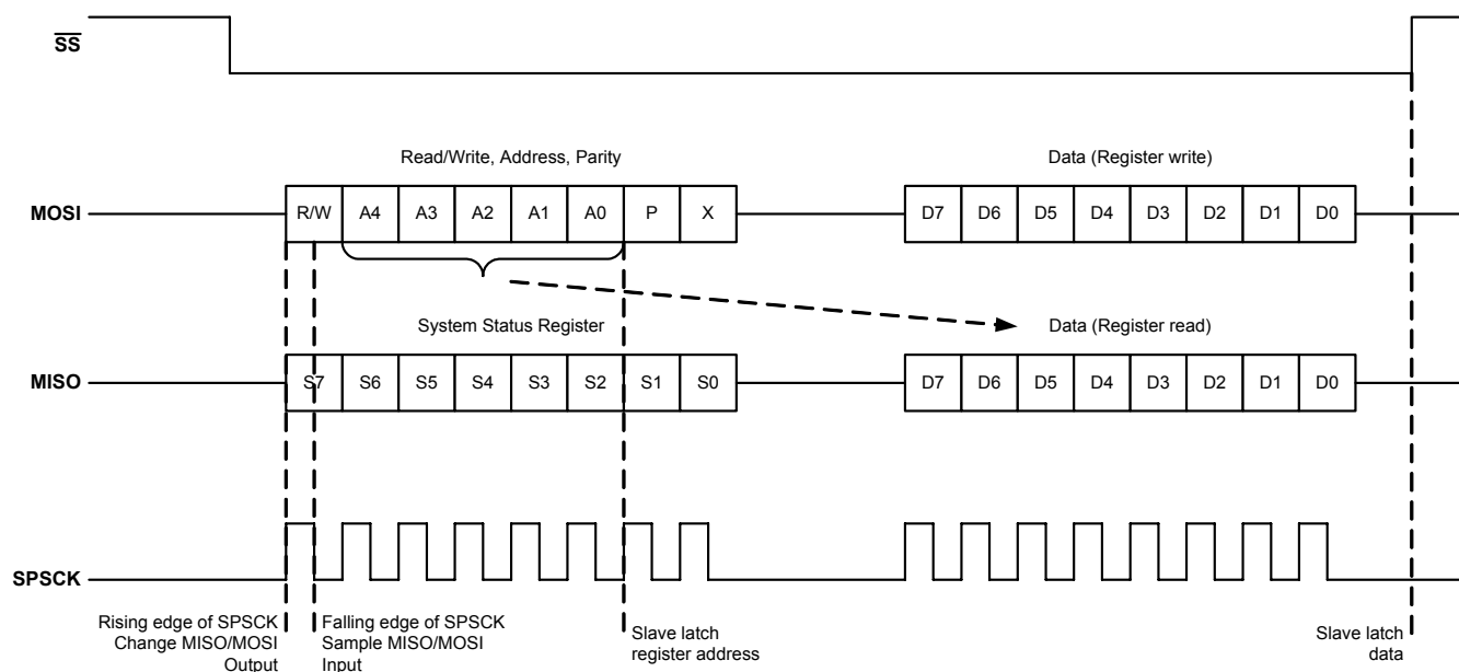
Figure 9. SPI Protocol
