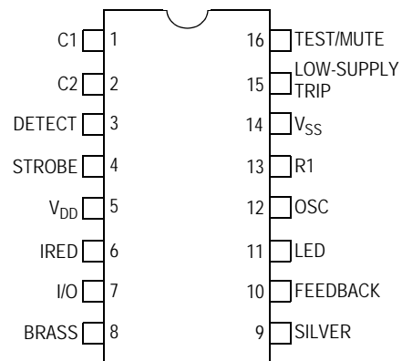
Figure 2. Pin Assignment (16-Pin DIP)
