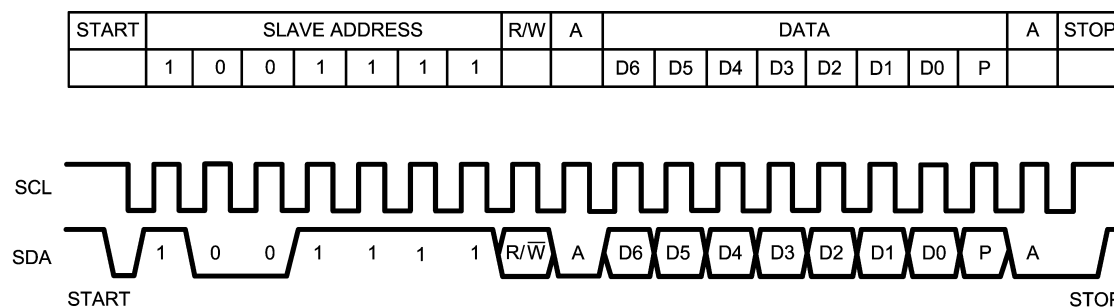
FIGURE 6. Timing Diagram
