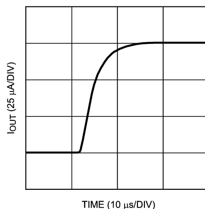
I_{OUT} Current Step Positive (Full Scale)
