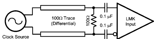
FIGURE 15. Differential Sine Wave Input
