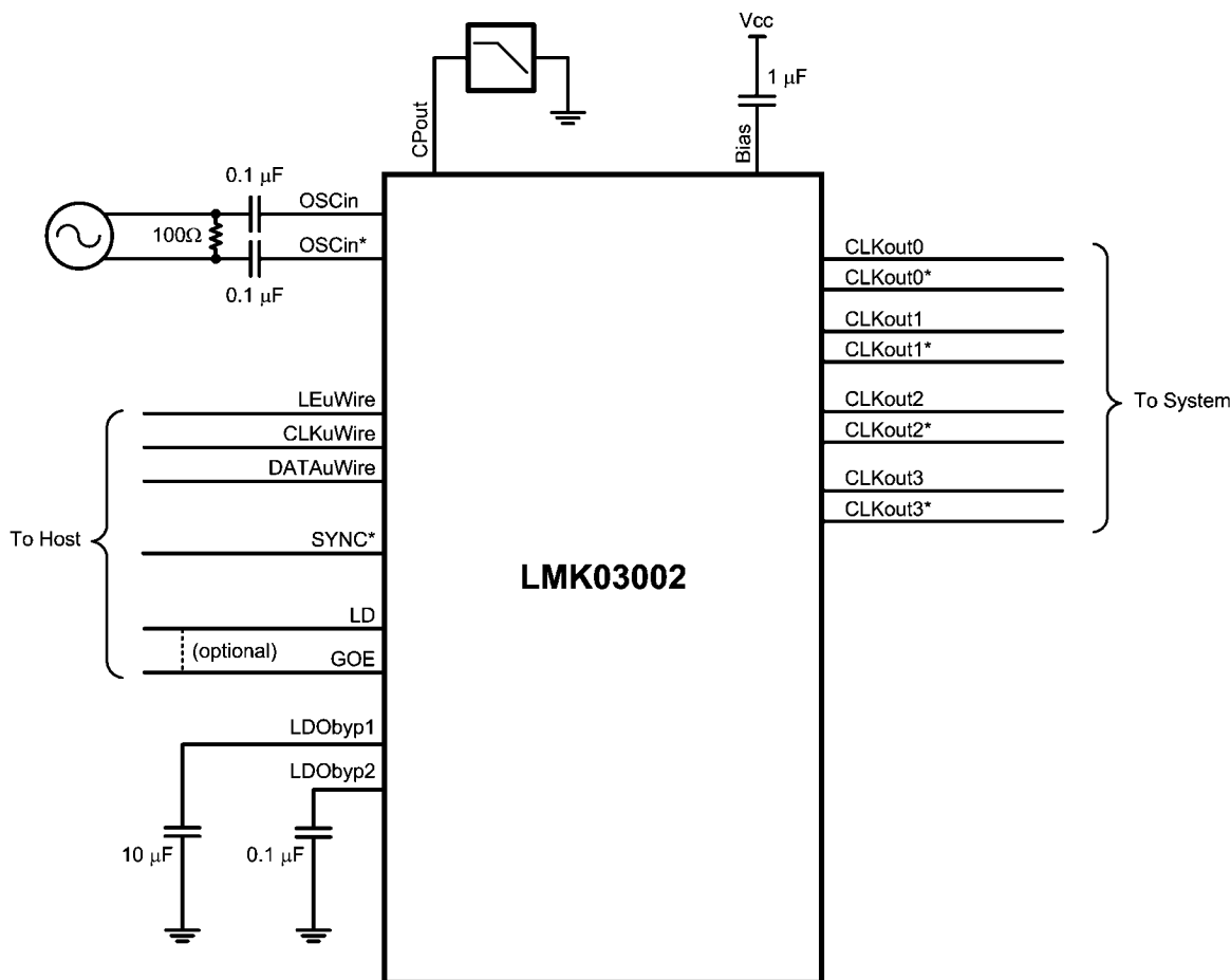
FIGURE 1. Typical Application
