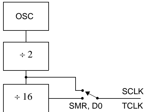
Figure 35. SCLK Circuit
