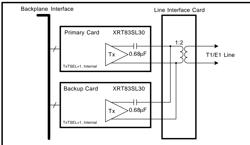
FIGURE 14. SIMPLIFIED BLOCK DIAGRAM OF THE TRANSMIT SECTION FOR 1:1 &amp; 1+1 REDUNDANCY
