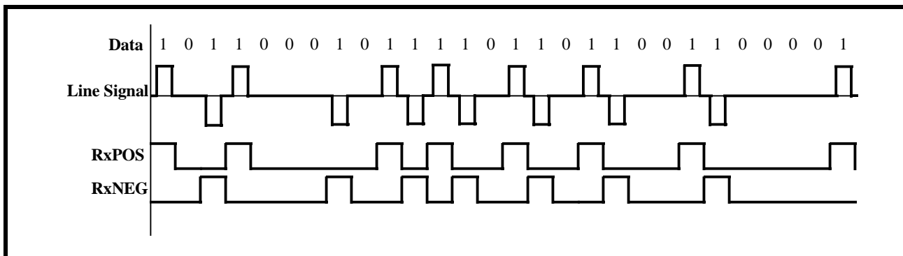
FIGURE 64. AMI LINE CODE
