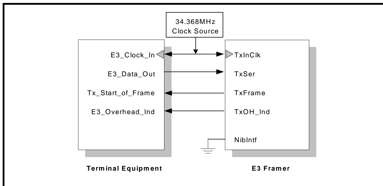
FIGURE 149. THE TERMINAL EQUIPMENT BEING INTERFACED TO THE TRANSMIT PAYLOAD DATA INPUT INTERFACE BLOCK FOR MODE 3 (SERIAL/LOCAL-TIMED/FRAME-MASTER) OPERATION
