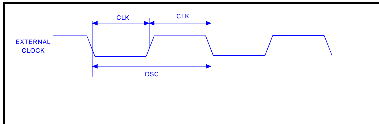
FIGURE 13. CLOCK TIMING
