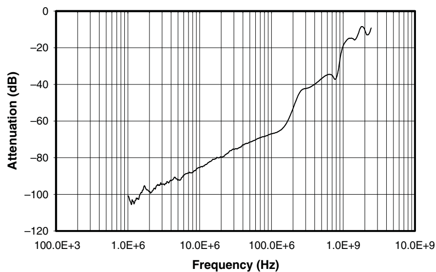
Figure 3. Crosstalk
