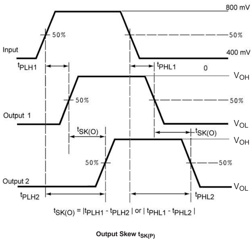
Figure 10. Skew Test
