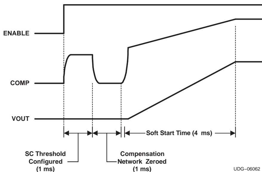
Figure 13. Startup Sequence
