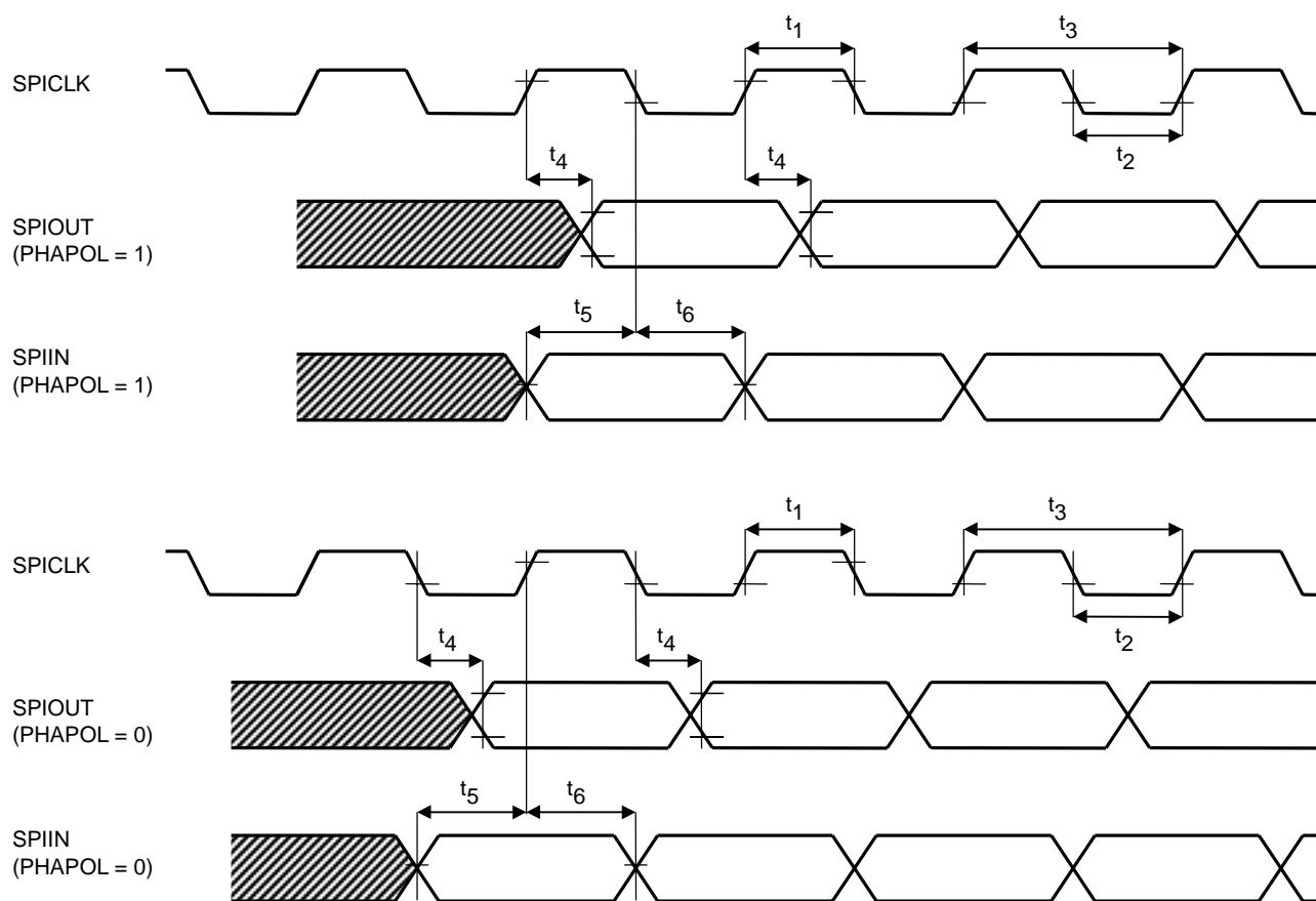
SPI Timing
