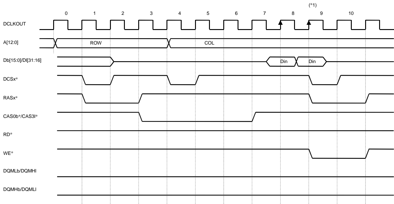
Figure B.73 16-bit SDRAM: Read Operation (1) (Byte/Halfword/Tripleword/Word)
