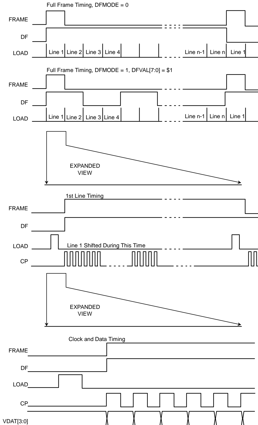
Figure 17.2.3 LCD Timing
