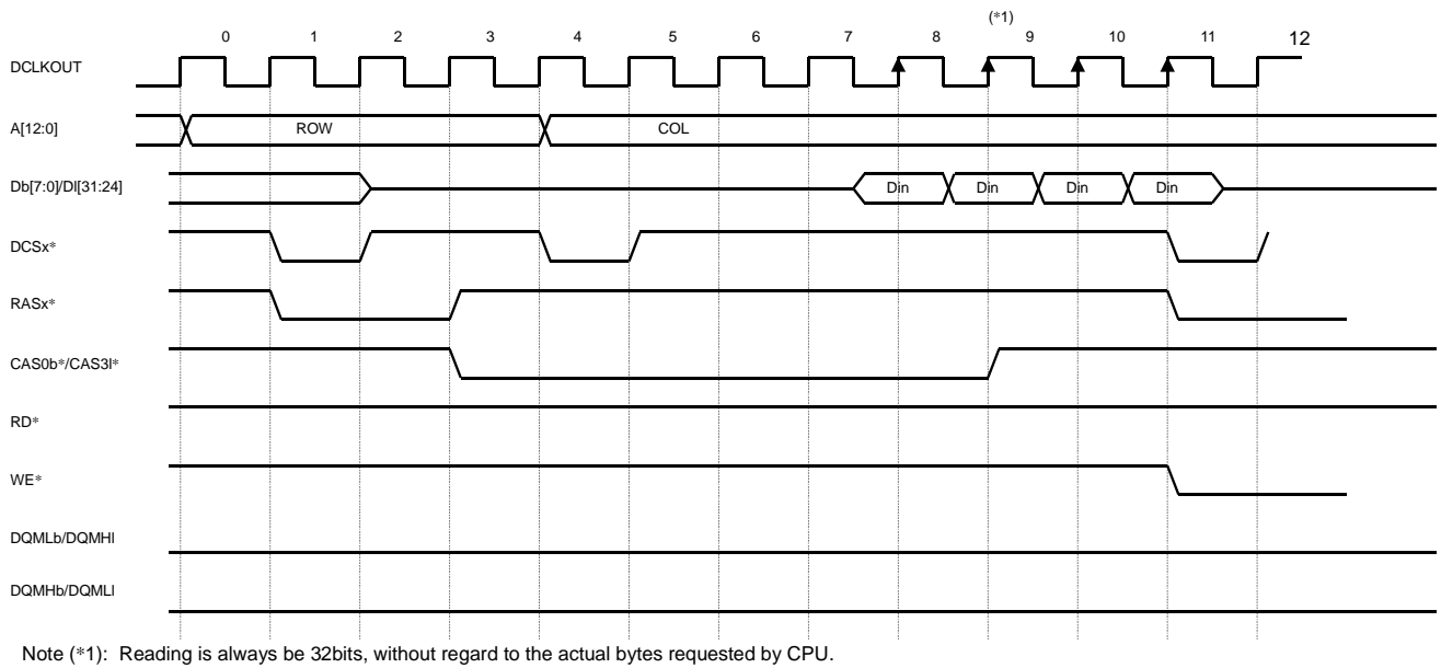
Figure B.66 8-bit SDRAM: Read Operation (1) (Byte/Halfword/Tripleword/Word)
