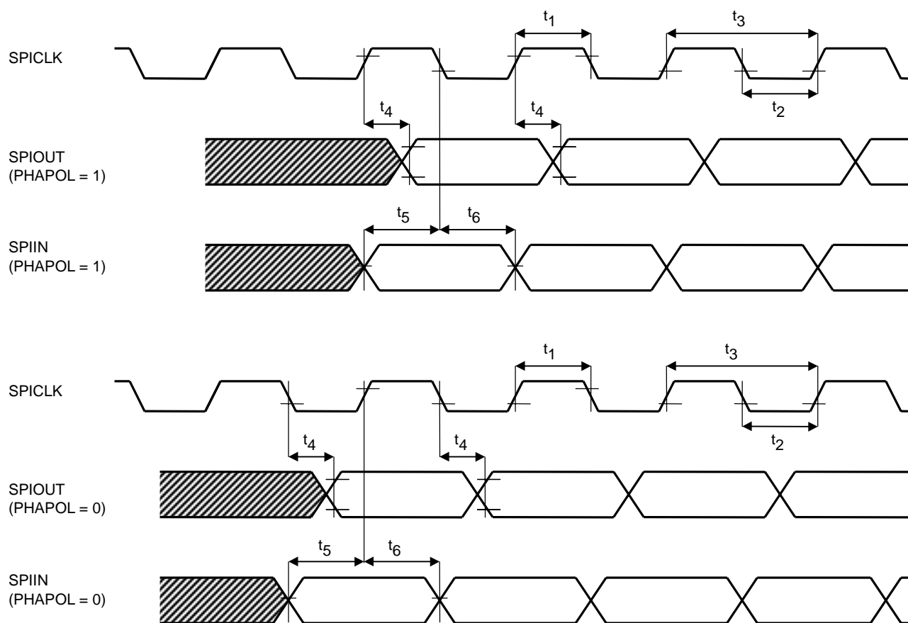
SPI Timing
