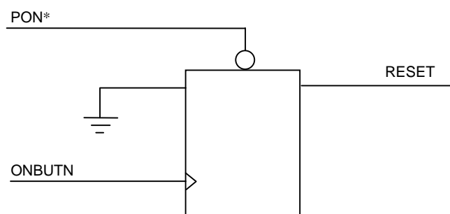
Figure 12.2.1 Reset Flip-Flop
