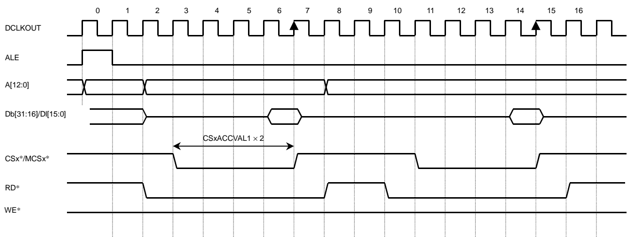
Figure B.7 16-bit Chip Select Device: Read Operation (3) (Triplebyte)
