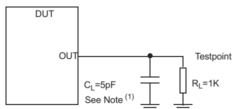
Figure 22 — Partial parity out load circuit
