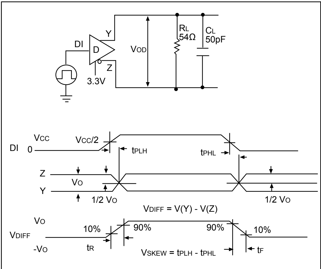
Figure 3. Driver Propagation Delay Time Test Circuit and Timing Diagram
