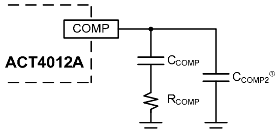
Stability Compensation
