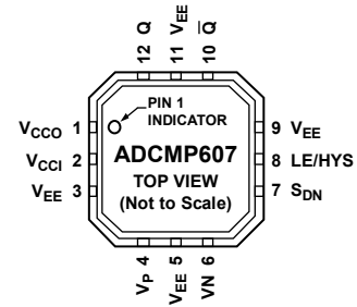
Figure 4. ADCMP607 Pin Configuration
