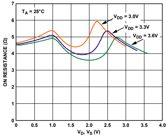
Figure 4. On Resistance vs. V_D ( V_S ) V_{DD} = 3.0\text{ V to } 3.6\text{ V}
