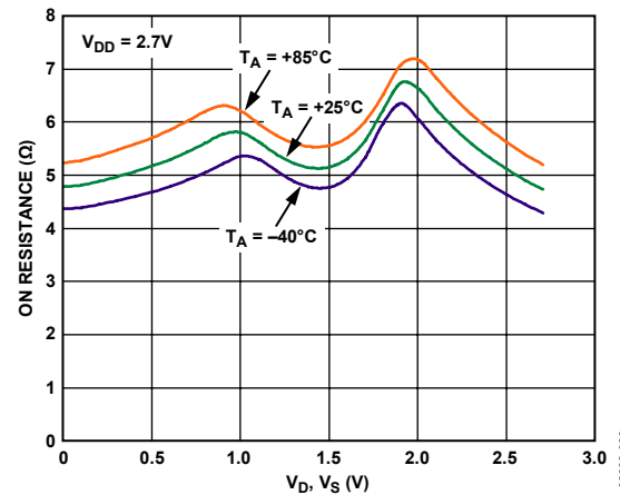
Figure 8. On Resistance vs. V_D ( V_S ) for Different Temperature, V_{DD} = 2.7\text{ V}
