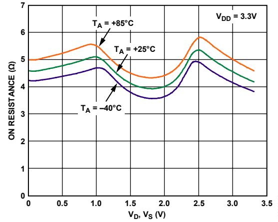
Figure 7. On Resistance vs. V_D ( V_S ) for Different Temperature, V_{DD} = 3.3\text{ V}
