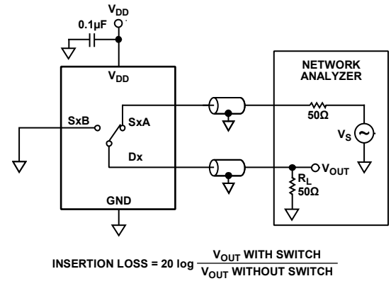
Figure 23. -3 dB Bandwidth
