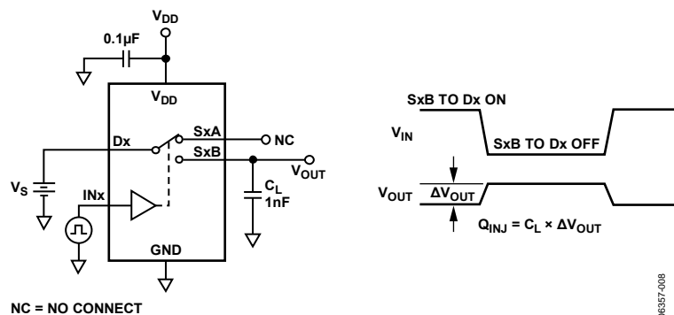
Figure 26. Charge Injection
