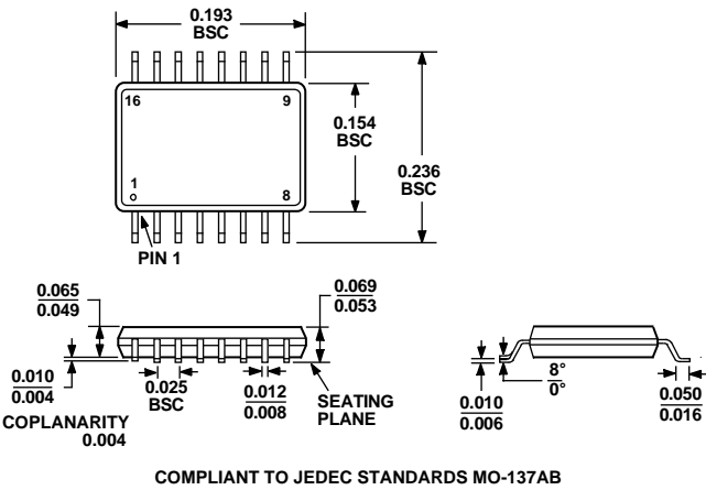
Figure 31. 16-Lead Shrink Small Outline Package [QSOP] (RQ-16) Dimensions shown in millimeters
