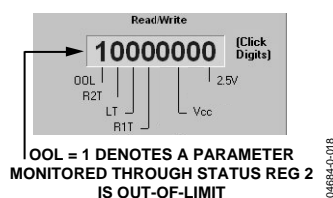
Figure 18. Interrupt Status Register 1
