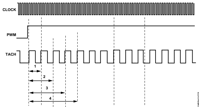
Figure 29. Fan Speed Measurement
