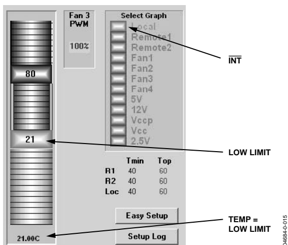
Figure 15. Temperature = Low Limit— \overline{\text{INT}} Occurs
