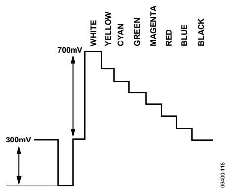
Figure 117. Y Levels—PAL
