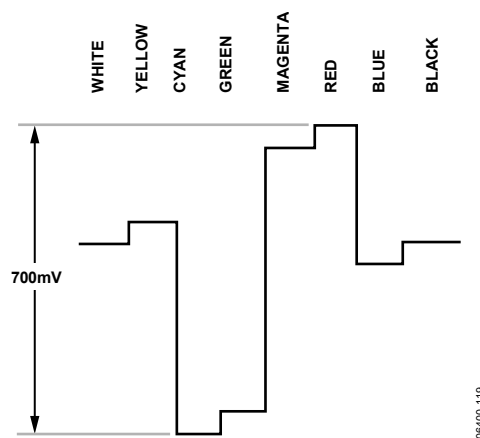
Figure 118. Pr Levels—PAL
