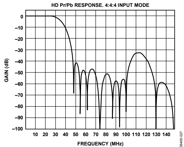
Figure 27. HD 4x Oversampling, Pr/Pb (SSAF) Filter Response (4:4:4 Input)
