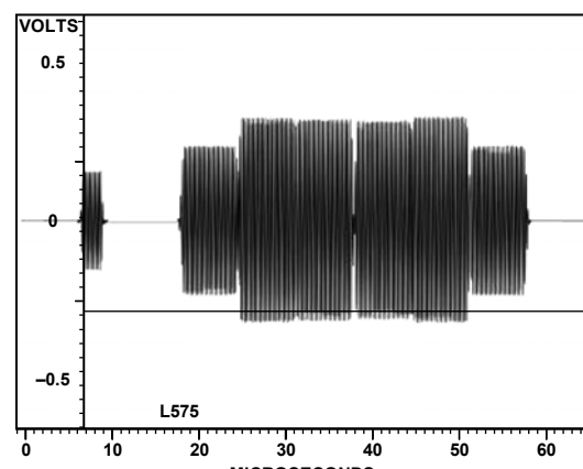
Figure 132. PAL Luma
