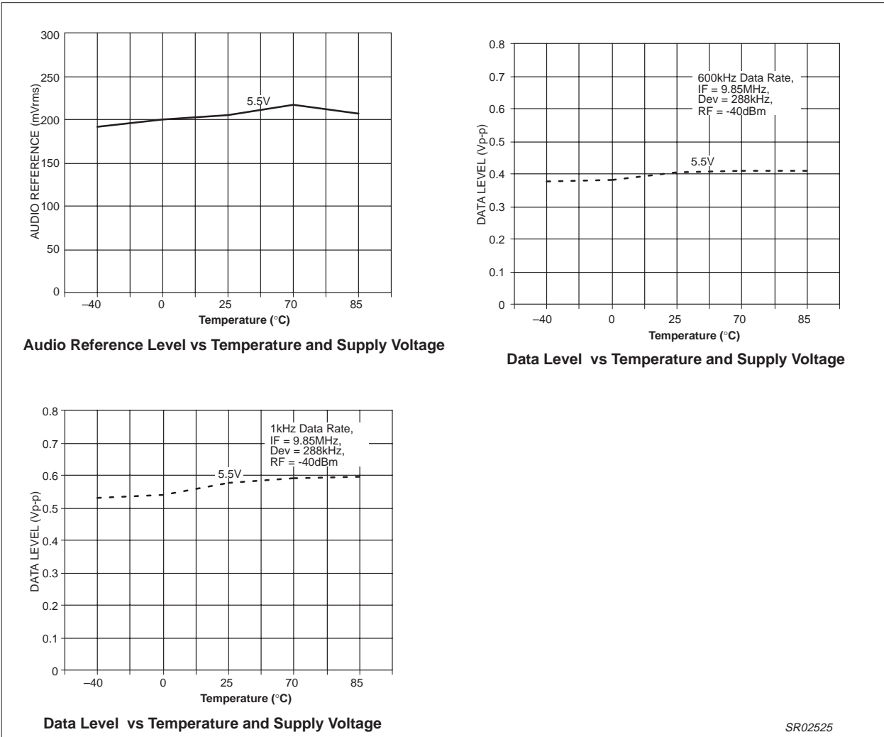
Figure 6. Performance Characteristics
