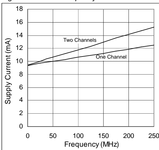
Figure 18. I_{CC} vs. Frequency
