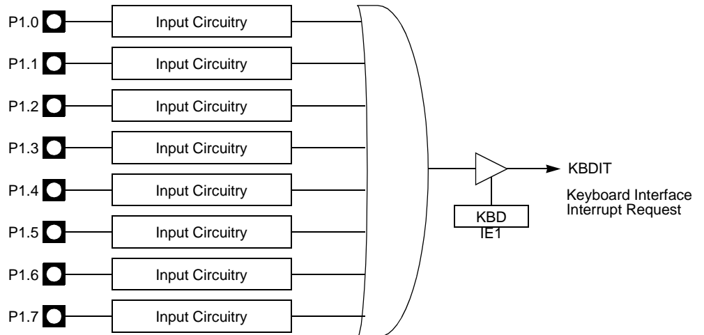
Figure 21. Keyboard Input Circuitry
