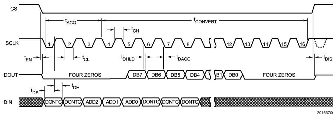
FIGURE 2. ADC088S022 Serial Timing Diagram
