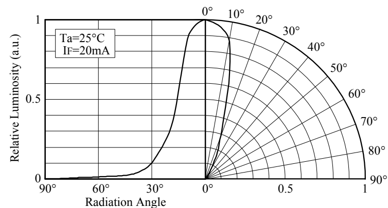
■ Directivity (NSPB510(S))
