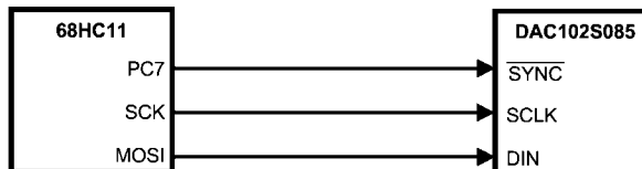
FIGURE 12. 68HC11 Interface
