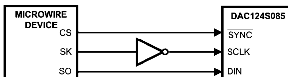
FIGURE 13. Microwire Interface
