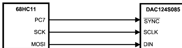
FIGURE 12. 68HC11 Interface
