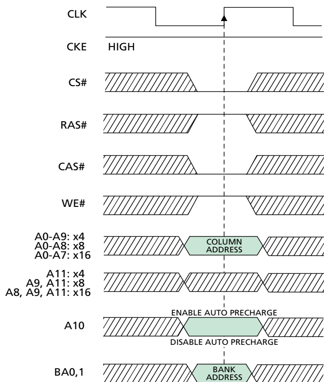
Figure 5 READ Command
