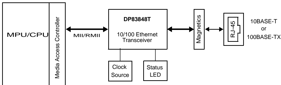
Typical Ethernet Application
