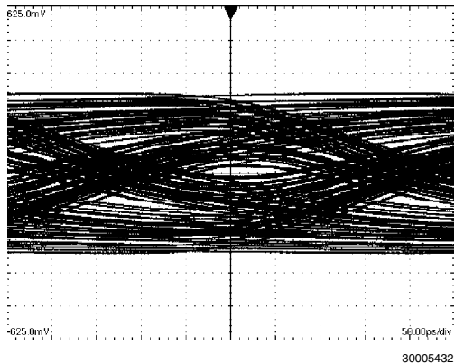
A 3.125 Gbps NRZ PRBS-7 After 40" Differential FR-4 Stripline V:125 mV / DIV, H:50 ps / DIV
