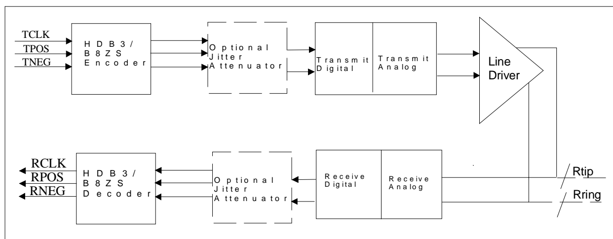
Figure 5-10. Analog Loopback
