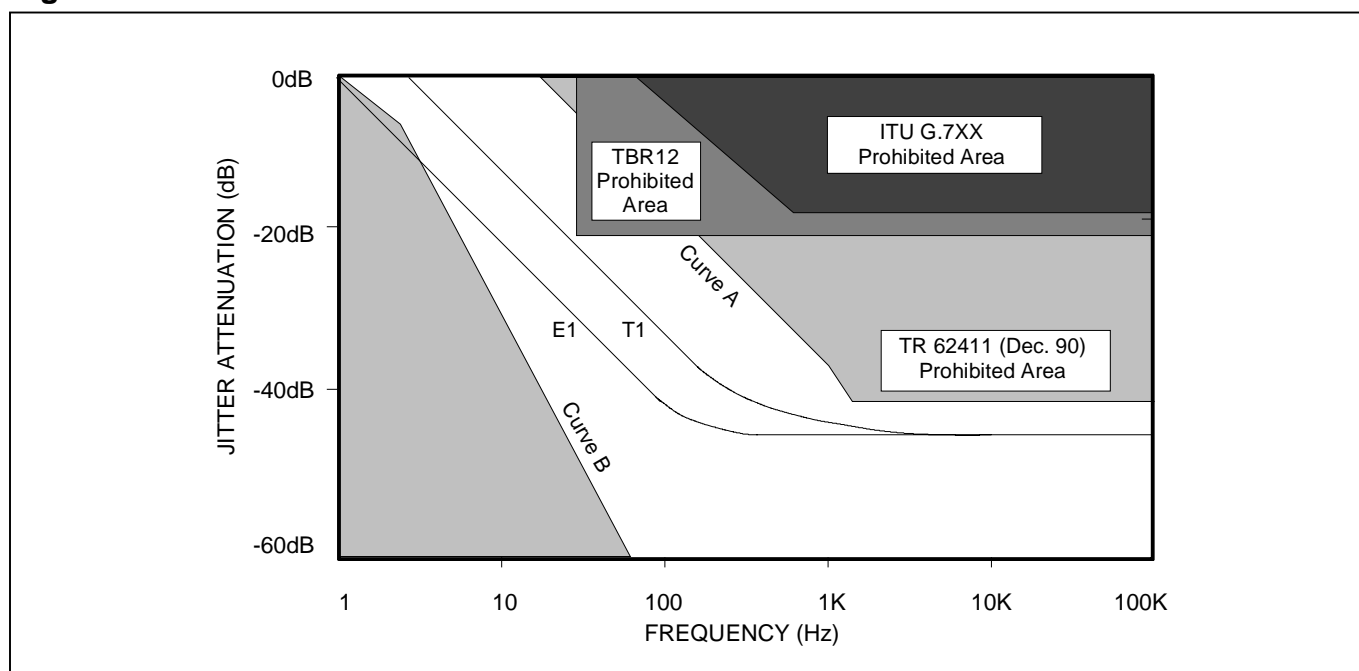
Figure 5-9. Jitter Attenuation
