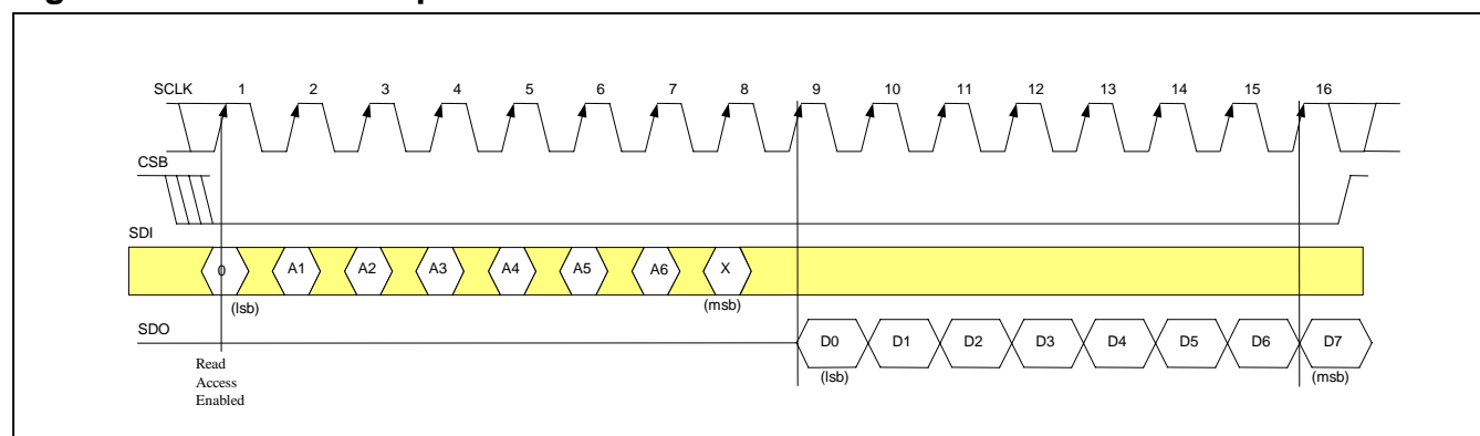
Figure 5-2. Serial Port Operation for Read Access with CLKE = 0
