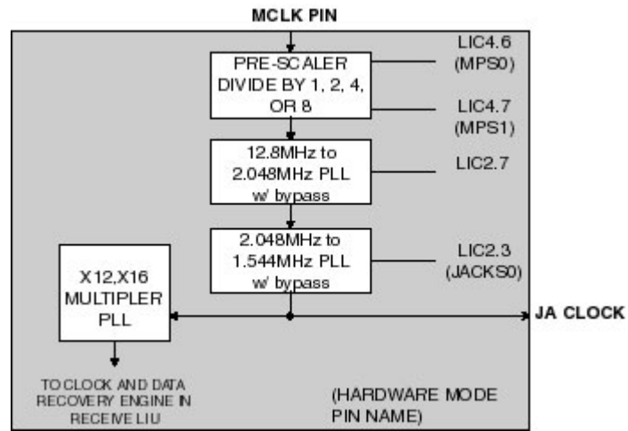
Figure 3-4. Master Clock PLL Diagram
