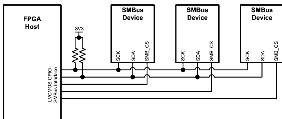
FIGURE 9. SMBus Configuration 2
