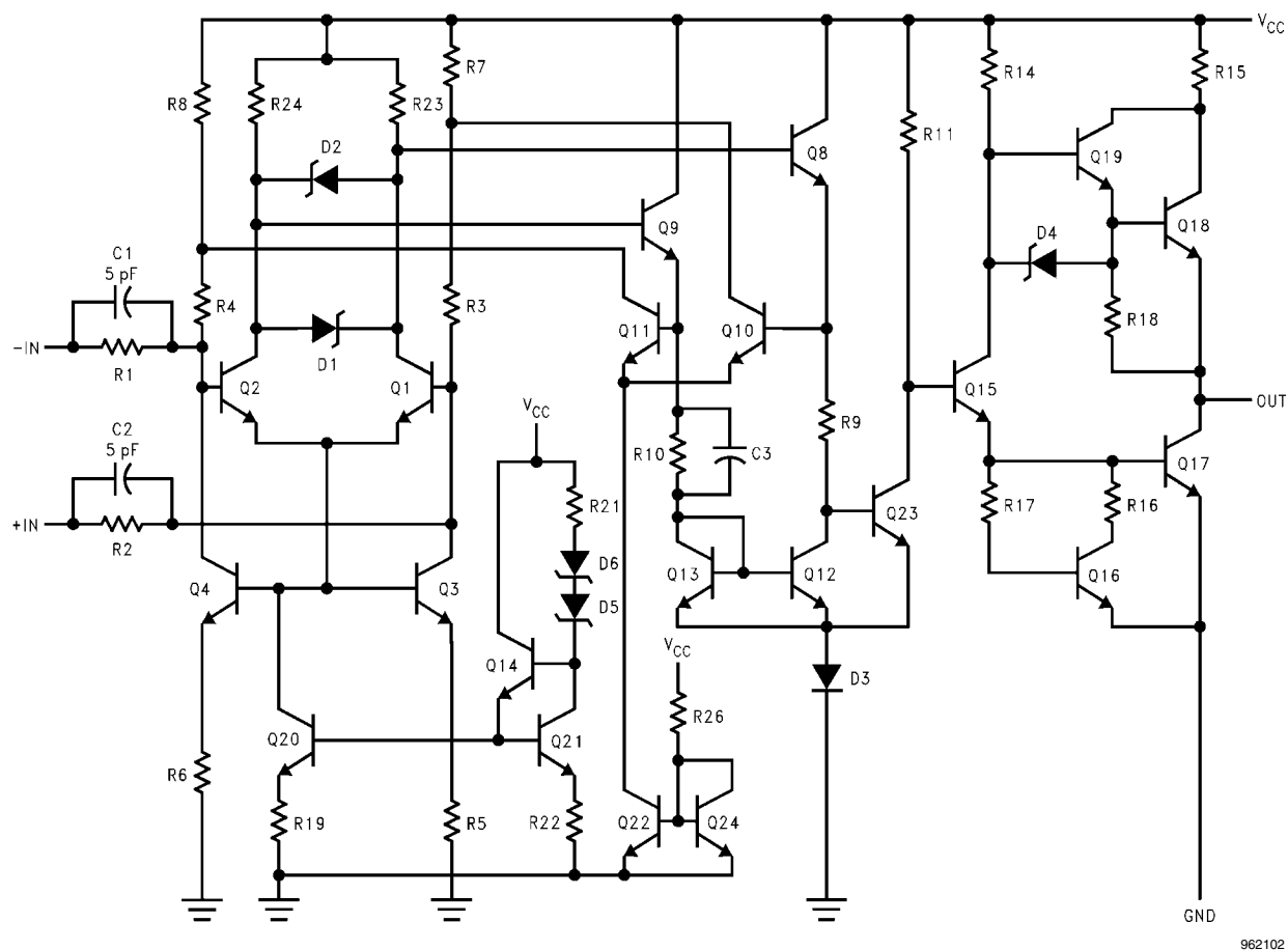
FIGURE 1. Equivalent Circuit
