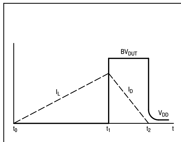
Figure 11. Current-Voltage Waveforms
