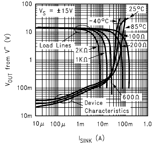
FIGURE 7. Output Sinking Characteristics with Load Lines
