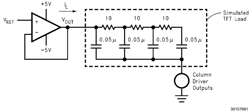
FIGURE 8. V_{COM} Driver Application Schematic
