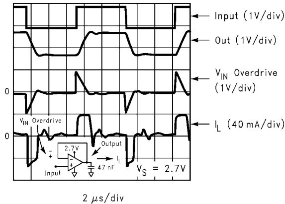
FIGURE 5. Buffer Amplifier scope photo
