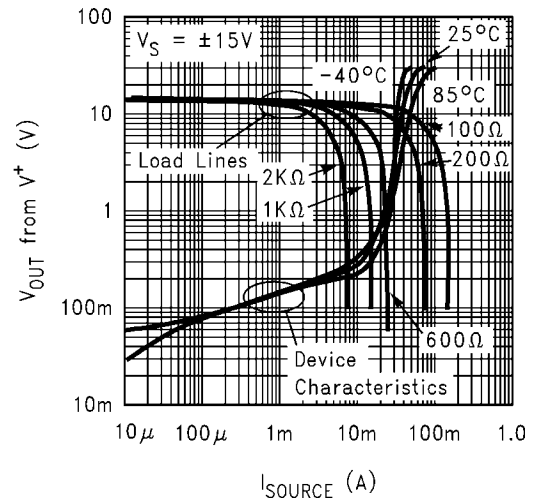
FIGURE 6. Output Sourcing Characteristics with Load Lines
