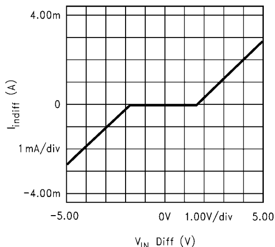
FIGURE 2. Input Stage Current vs. Differential Input Voltage
