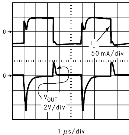
FIGURE 9. V_{COM} driver performance scope photo
