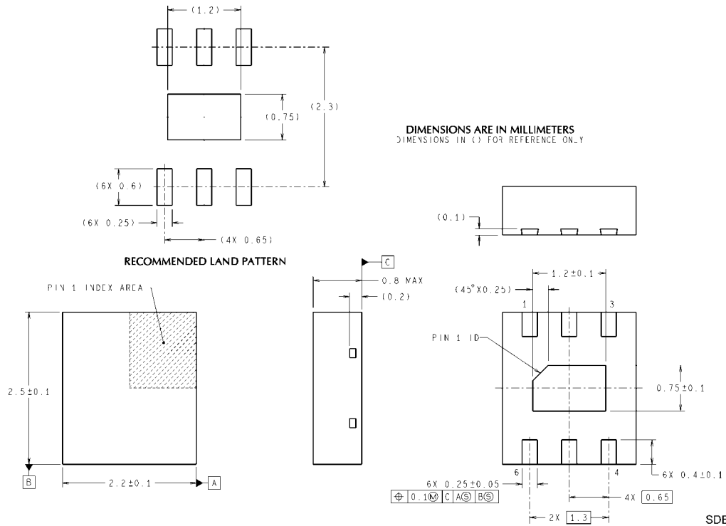
6-Lead LLP-6 Package NS Package Number SDB06A
